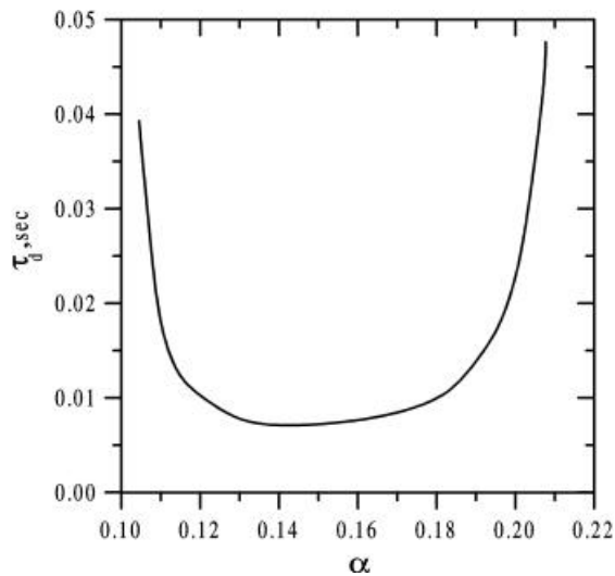
Fig. 2. The diffusion time versus the pitch parameter \alpha \equiv E / n\mathbf{B} - 1 at r = 0.5a in a Helias reactor with \mathbf{b} = 4.7\% .
