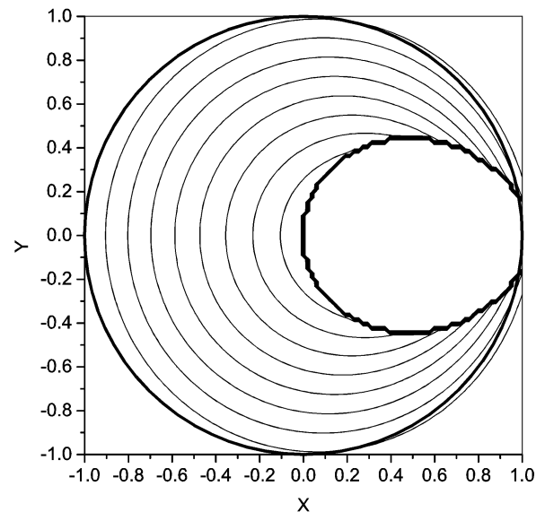
Fig. 1. Sketch of level contours of J for the locally trapped particles (thin lines) and the \mathbf{k} = 1 contour (bold line inside the plasma) in a Helias. Locally trapped particles moving along the J_1 = \text{const} contours become locally passing ones after crossing the bold line.
