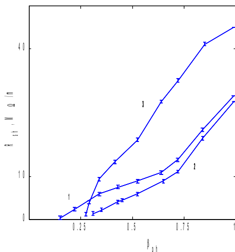
Fig. 1. Shunt impedance of wave dielectric structure vs phase velocity of wave.
