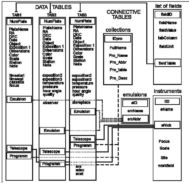
Figure 1. The structure of database
