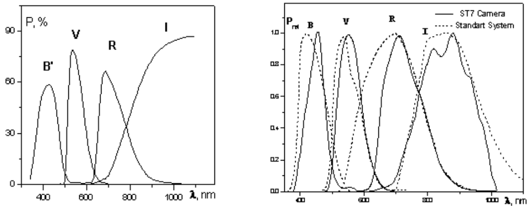
Figure 1. Transparency of the filter set (left) and the normalized filters curves of spectral transparency of the ST7 camera (right)
