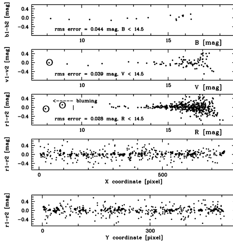
Figure 2. Test of instrumental photometric accuracy of the CCD ST7 camera
