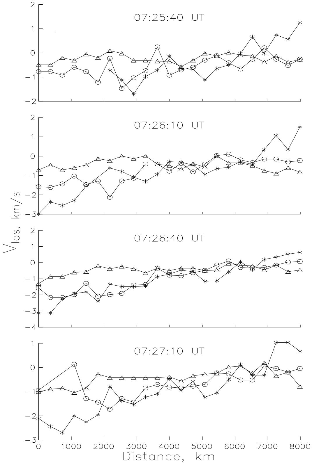
Figure 1. Variations of photospheric line-of-sight velocities derived from the Fe I \lambda 630.25 nm line (triangles), the Fe I \lambda 630.35 nm line (asterisks), and the Ti I \lambda 630.38 nm line (circles) on the plage surface at 07:25:40–07:27:10 UT. Positive values represent the motion from an observer. Vertical bar is the observational error of the velocity
