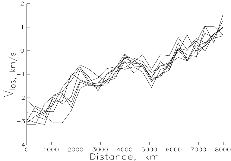
Figure 3. Variations of photospheric line-of-sight velocities derived from the FeI \lambda 630.25 nm line on the plage surface at all moments of the observation
