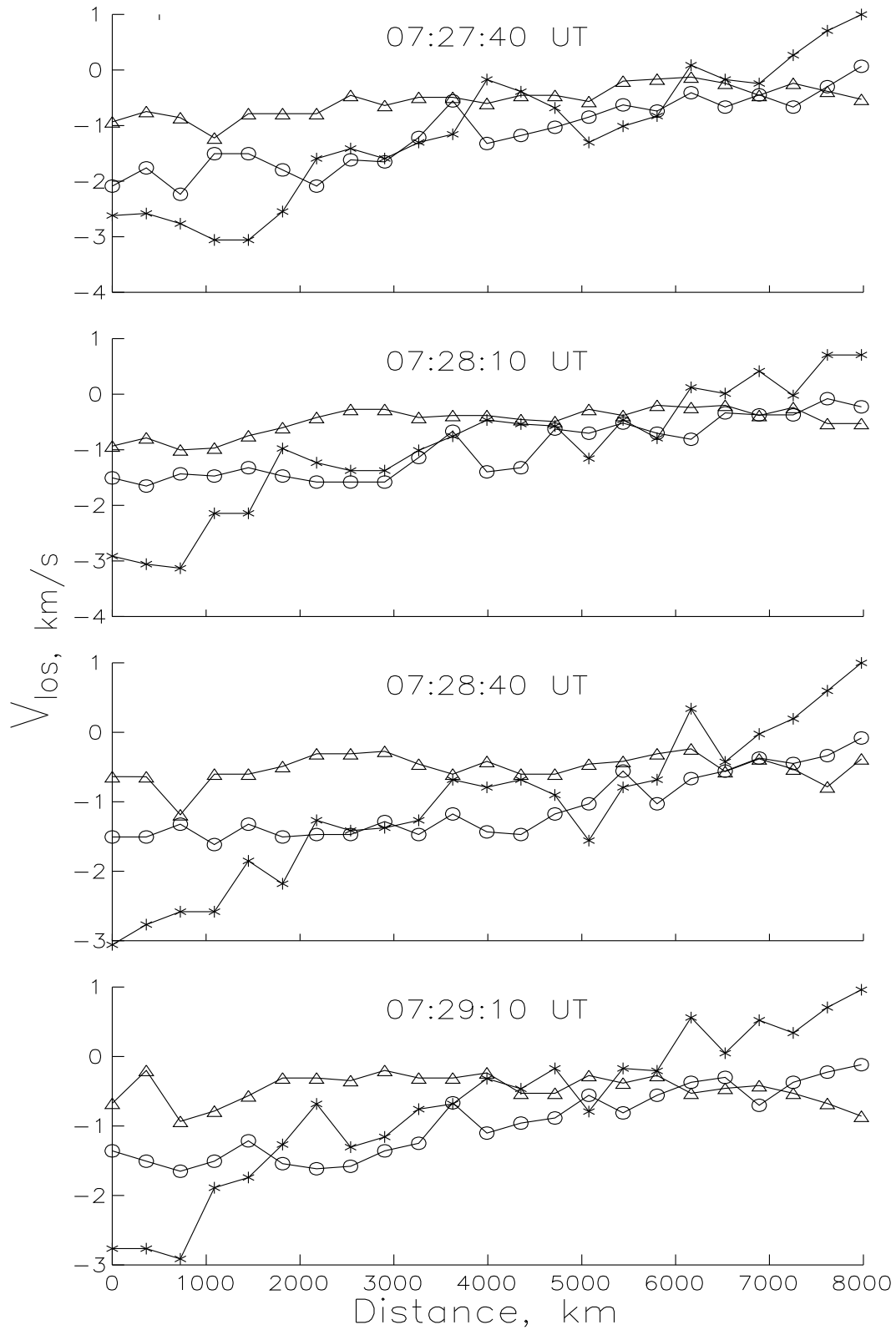
Figure 2. The same as Fig. 1 at 07:27:40–07:29:10 UT
