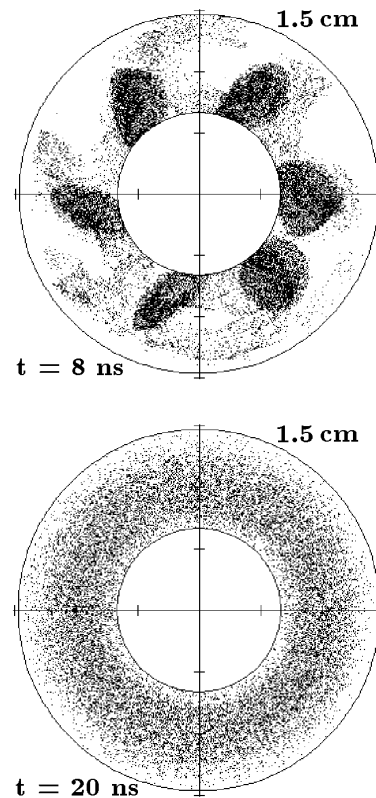
Fig. 2. Configurations of flow at t = 8 ns and t = 20 ns
