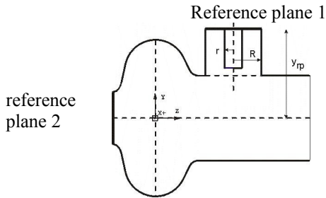
Fig. 4. Input coupler model with reference planes positions showed.
