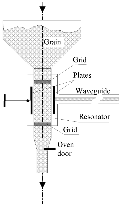
Fig. 1. Sketch of the treatment device.
