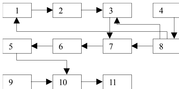
Fig. 4. The simplified block-diagram of the installation: 1 - power transformer, 2 - AC/DC convertor, 3 - timing device, 4 - RF generator, 5 - pulse output transformer, 6 - artificial line, 7 - signalling and interlock, 8 - reception facility, 9 - device of a grain treatment, 10 - grain reception.
