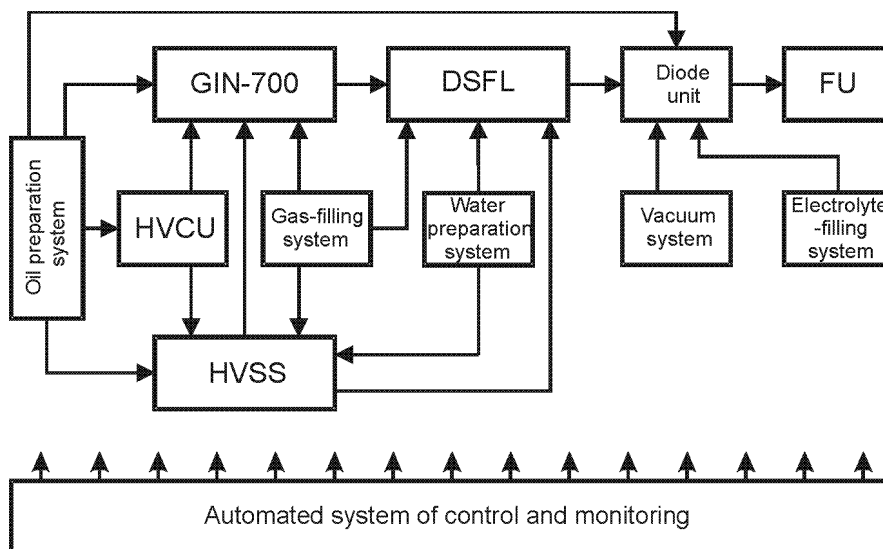
Fig. 1. Structural scheme of STRAUS-R accelerator.
