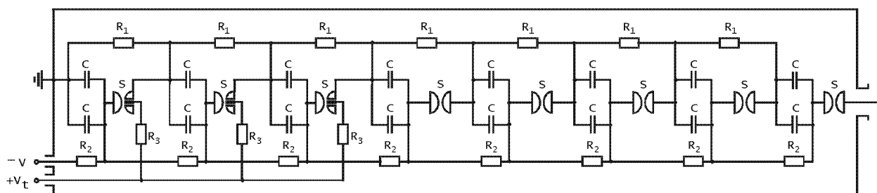
Fig. 3. Electrical circuit of GIN-700 generator.
