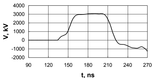
Fig. 4. Calculated diode voltage pulse of STRAUS-R accelerator.
