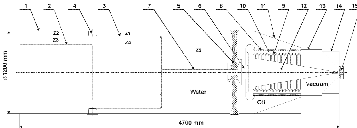
Fig. 2. Structural scheme of STRAUS-R forming system and diode unit.
