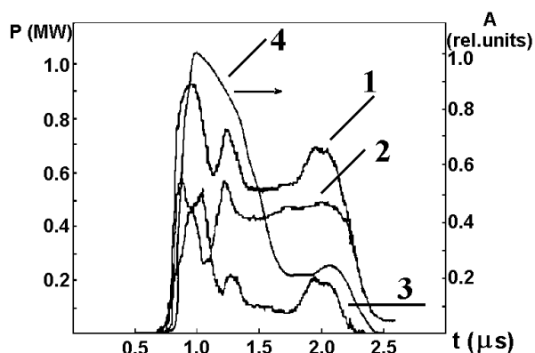
Fig. 2. Time dependence of the incident wave power (1), reflected wave power (2), power absorbed in a resonator (3) and the X-radiation intensity (4).
