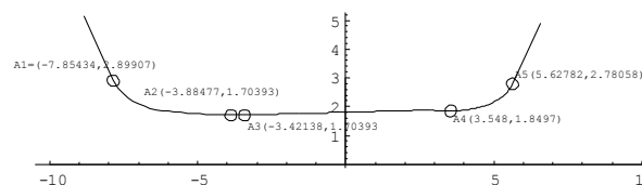
Fig. 2. Pole shape in a regular part of the magnet.
