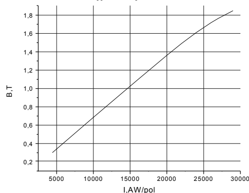
Fig. 6. A magnetization curve of a magnet.
