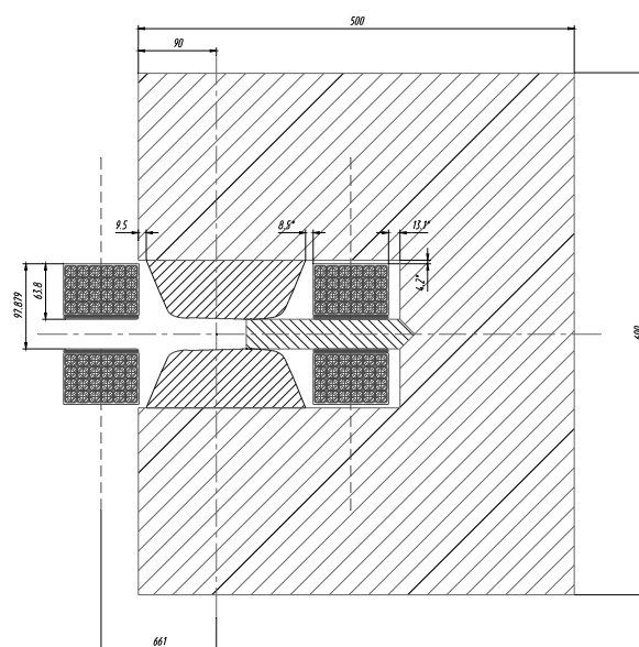
Fig. 1. Cross section of dipole magnet.
