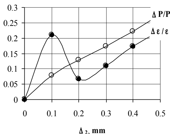
Fig. 3. Relative deviations of the emittance – \Delta\varepsilon/\varepsilon
