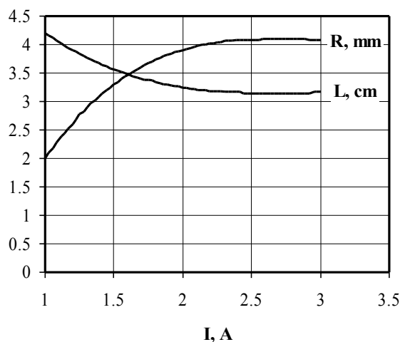
Fig. 5. Position of crossover L and beam radius in the crossover vs emission ability of cathode I.
