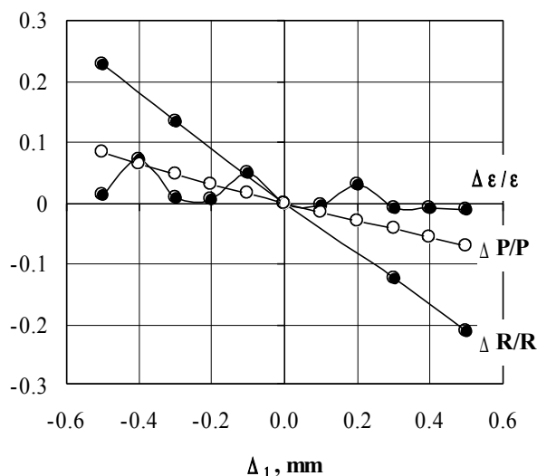
Fig. 2. Relative variations of emittance – \Delta\varepsilon/\varepsilon , perveance – \Delta P/P and the beam radius – \Delta R/R vs the anode displacement \Delta_1 .
