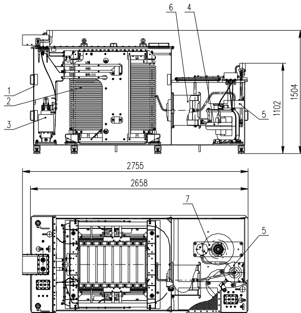
Fig. 5. PT design.
