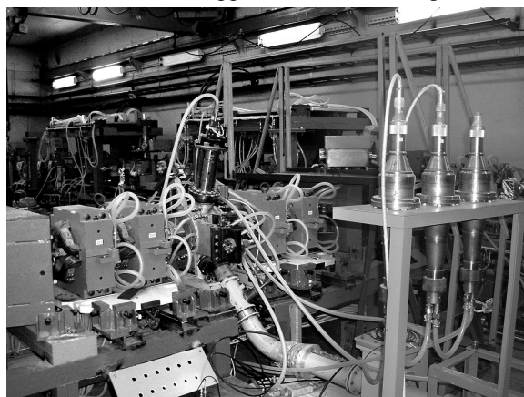
Fig.2. RF cavity in the damping ring
