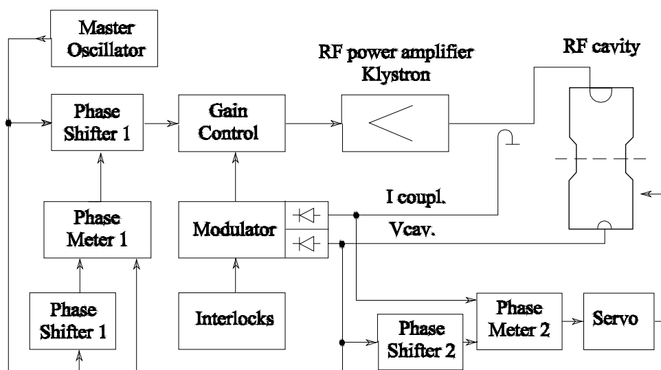
Fig.3. RF control system block diagram
