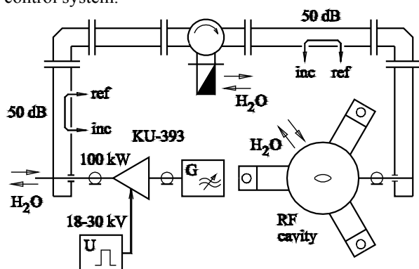
Fig.1. RF system block diagram
