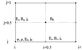
Fig. 1. Fragment of space mesh with field components.
