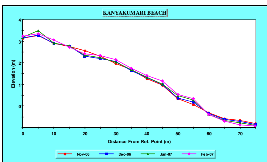
Fig. 6. Post-Monsoon Profiles of Kanyakumari Beach
