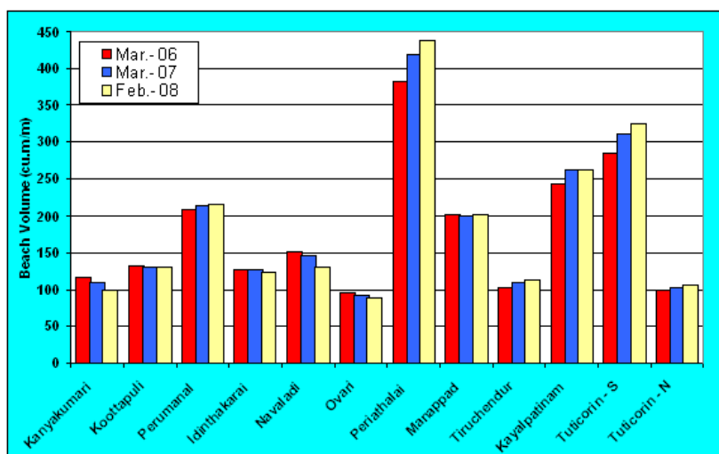
Fig. 9. Annual Variation of Sediment Volume
