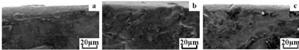
Fig. 4. SEM micrographs showing crack initiation site in laboratory air ( \sigma = 110 MPa): (a) AZ80, (b) AZ61, (c) AM60.
