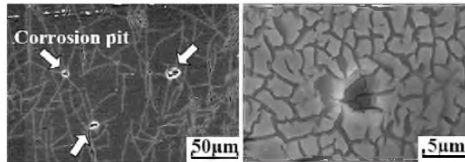
Fig. 8. Specimen surfaces of AM60 ( \sigma = 50 MPa).
