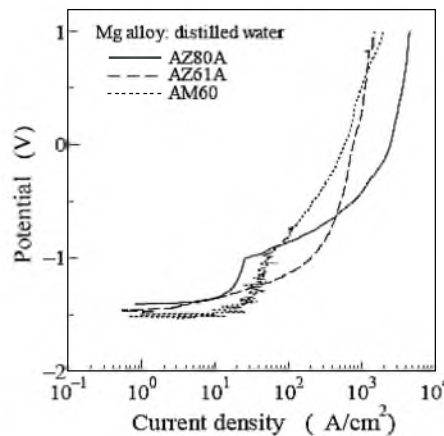
Fig. 9. Anode polarization curves in distilled water.
