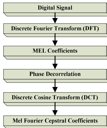
Fig. 2. Obtaining the MFCCs
