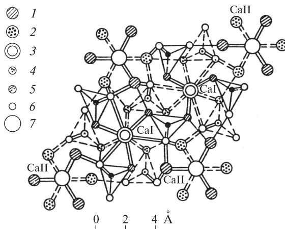
Fig. 6. Fluorapatite structure: 1 — Ca on \frac{1}{4}c ; 2 — Ca on \frac{3}{4}c ; 3 — Ca on 0, \frac{1}{2}c ; 4 — O on \frac{3}{4}c ; 5 — O on \frac{1}{4}c ; 6 — O on \frac{1}{20}, \frac{3}{20}c etc.; 7 — F on \frac{1}{4}, \frac{3}{4}c .
