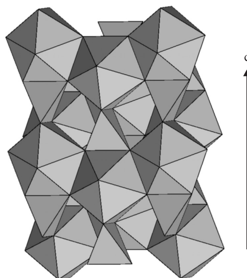
Fig. 3. Zircon structure
