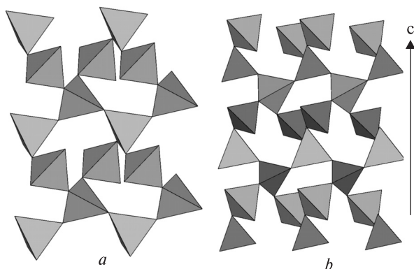
Fig. 4. Quartz (a) and gallium phosphate (b) structures
