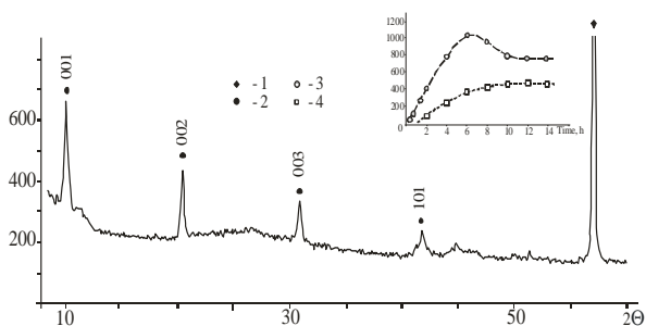
Fig. 1. XRD data of hydroxysulfate Green Rust II (GR(SO 4 2- )) sample: 1 – α-Fe 0 , 2 – GR(SO 4 2- ); the kinetic of reflection intensity the planes of GR(SO 4 2- ): 3 – (001), 4 – (002) on the additional graph
