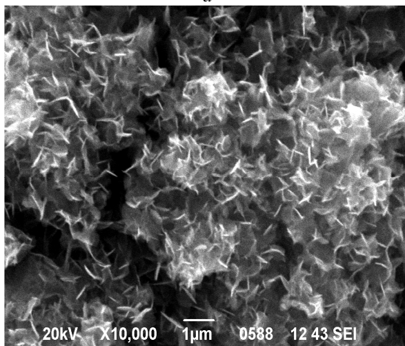
Fig. 2. Structures of Fe (II)–Fe (III) layered double hydroxide (GR(SO 4 2- )) formed on the surface of steel electrode by its contact with water dispersion medium at free access of air oxygen into the system
