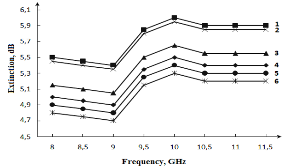
Fig. 2. Frequency dependence of the extinction of electromagnetic radiation as it passes through \text{SiO}_2 based materials with different magnetic fillers: □ – \text{BaFe}_{12}\text{O}_{19}+\alpha\text{-Fe}_2\text{O}_3 ; x – \text{BaFe}_{12}\text{O}_{19}+\text{Zn} ; △ – \text{BaFe}_{12}\text{O}_{19} ; ◇ – \text{BaFe}_{12}\text{O}_{19}+\alpha\text{-Fe}_2\text{O}_3 (Peccini's method); ○ – \text{SrFe}_{12}\text{O}_{19} (with dope); * – \text{SrFe}_{12}\text{O}_{19}
