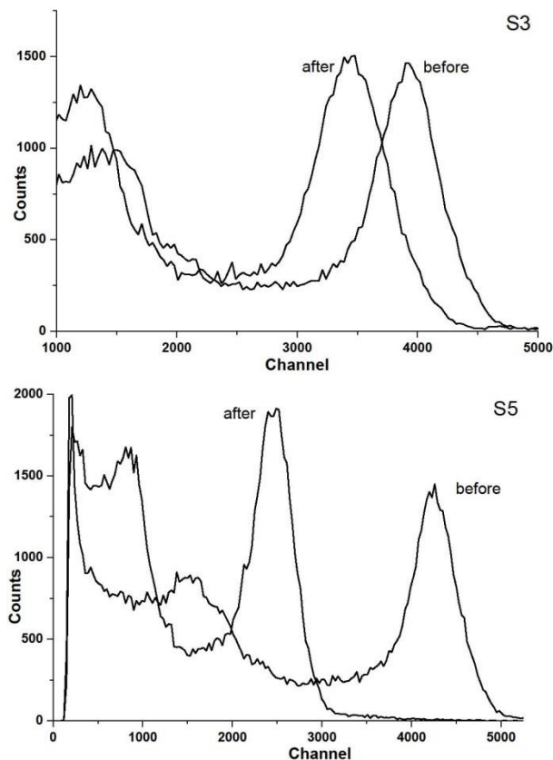
Fig. 5. Scintillation amplitude spectra of PS samples S3 and S5 before and after irradiation with a dose of 10 Mrad
