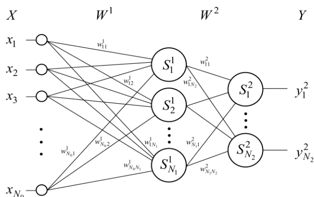
FIG. 2. Multilayer network
