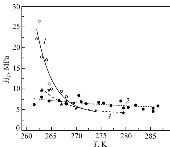
Fig. 4. The temperature dependences of microhardness of the epoxy resin: single-wall carbon nanotubes+copolymer composite (CCS) (curves 1, 2; curve 2 was obtained a week later) and pure epoxy resin (ER) (curve 3). P = 0.01 N, t = 10 s.
