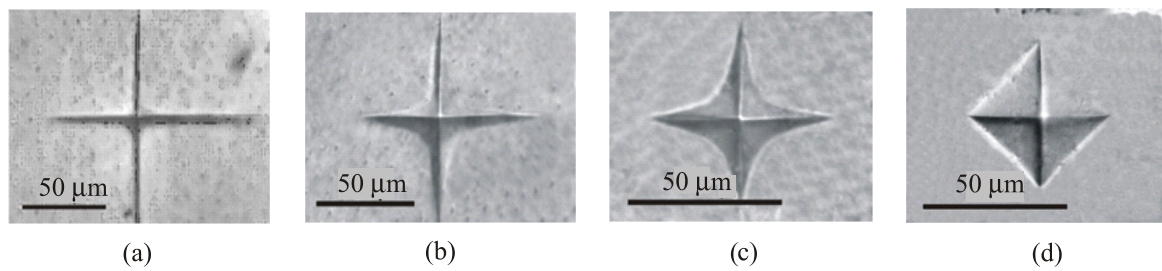
Fig. 3. Changes in the form of impressions at lowering temperature, K: 280 (a), 275 (b), 271 (c), 265 (d). Load P = 0.05 N, loading duration t = 10 s.
