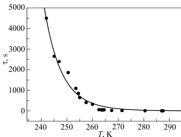
Fig. 7. The temperature dependence of the relaxation time \tau(T) : the points indicate the values obtained by the substitution in the formula (14) the H_V values from Fig. 6 at \Delta t = 10 s; the solid line represents Eq. (9) using \tau_0 = 10^{-12} s and U = 0.75 eV (8720 K in the temperature units).
