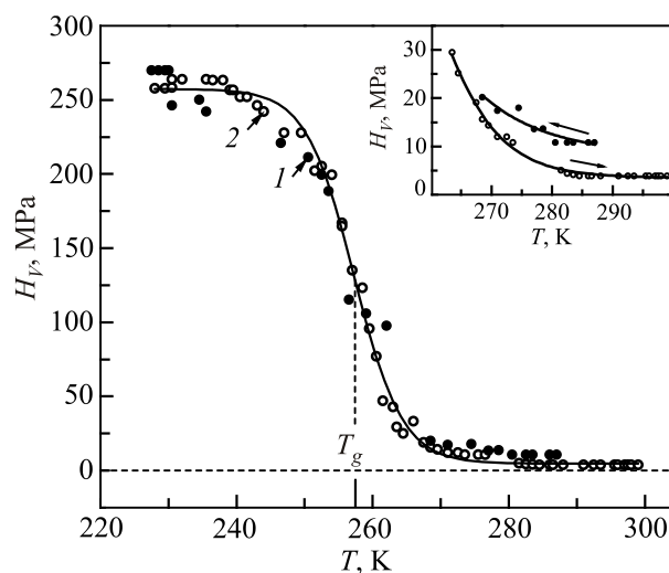
Fig. 5. The temperature dependences of microhardness H_V(T) of elastomer CE obtained on cooling (1) and heating (2) at P = 0.05 N and \Delta t = 10 s. In the insert: temperature hysteresis of the dependence close to the high-elastic region.
