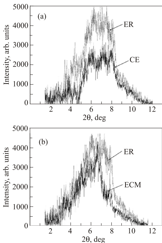
Fig. 1. Small-angle scattering from ER and CE (a) and ER and ECM (b) samples.
