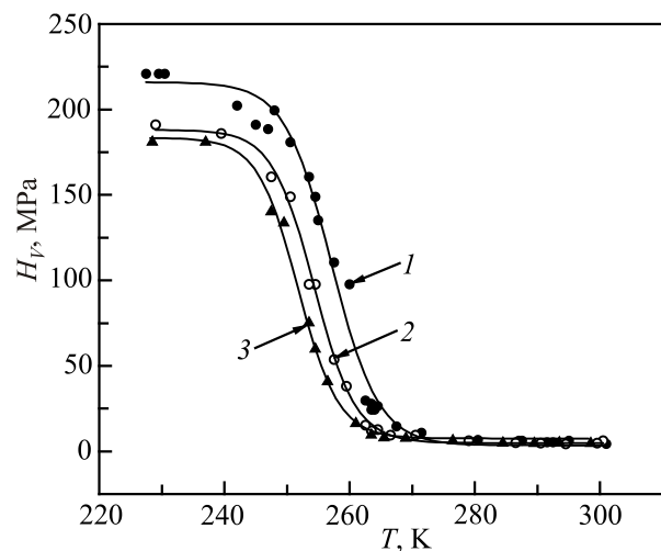
Fig. 6. The temperature dependences of microhardness of elastomer CE at P = 0.05\text{ N} and three values of the indentation duration: \Delta t = 10 (1), 30 (2) и 60 (3) s.
