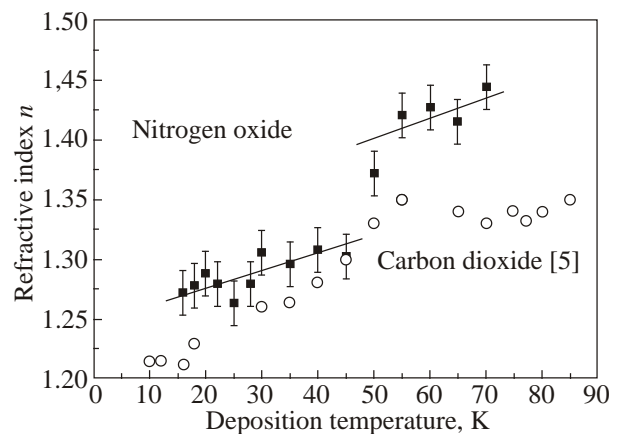
Fig. 2. Influence of deposition temperature on the refractive indices of nitrous oxide. For comparison, data for carbon dioxide are shown [5].
