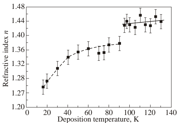
Fig. 1. Influence of deposition temperature on the refractive index of ethanol.
