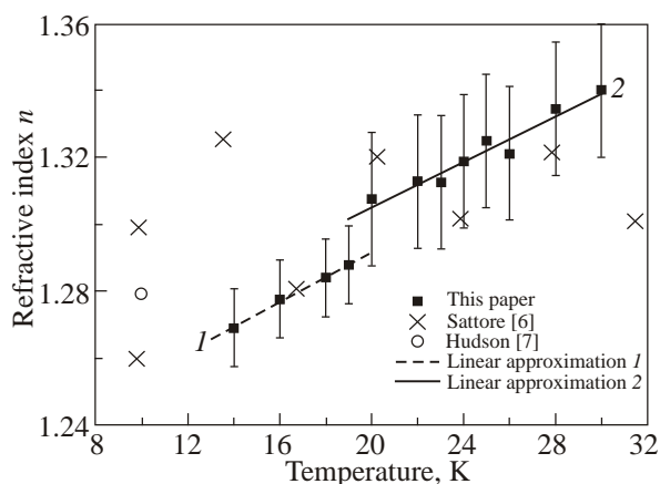
Fig. 3. Influence of deposition temperature on the refractive index of methane.
