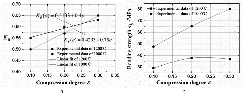
Fig. 6. Experimental results of high temperature bonding strength for bonding interface: (a) K_B(\epsilon) changes with rolling reduction; (b) \sigma_b changes with rolling reduction \epsilon .
