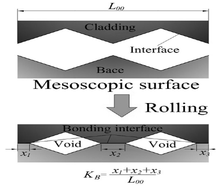
Fig. 3. Schematic diagram for interfacial bonding process at mesoscale.
