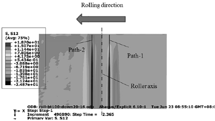
Fig. 8. Shear stress distribution of bonding interface during the rolling process.
