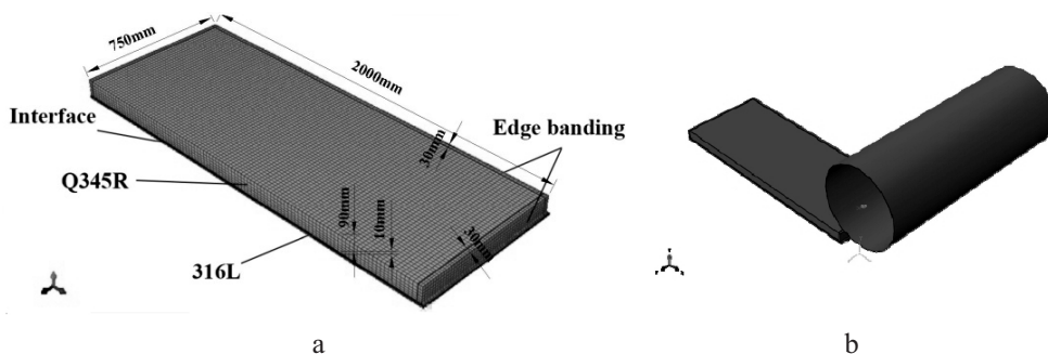
Fig. 7. Finite element rolling model: (a) finite element grid; (b) rolling process model.
