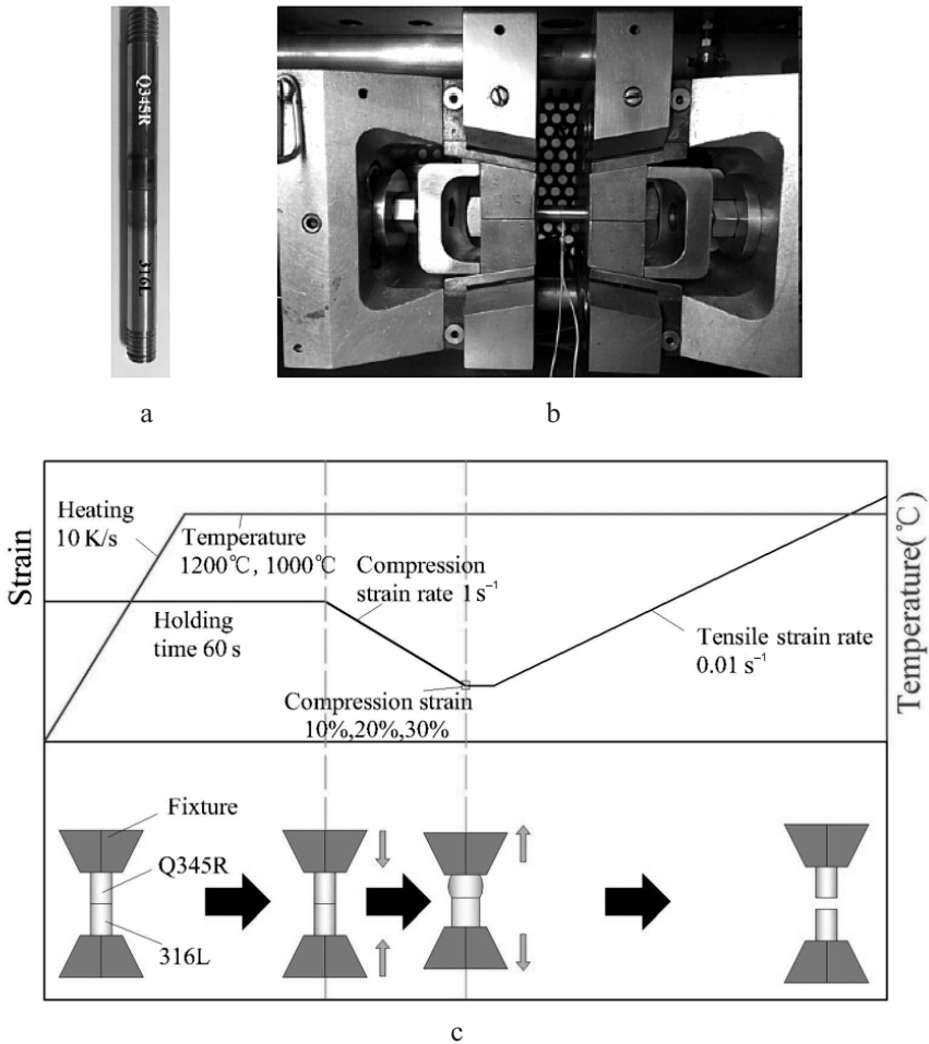
Fig. 5. Experiment of bonding strength of high temperature bonding interface: (a) specimen; (b) specimen clamping; (c) schematic diagram of the experimental process.
