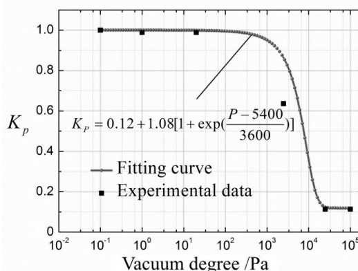
Fig. 2. Effect of vacuum depth on interfacial strength.
