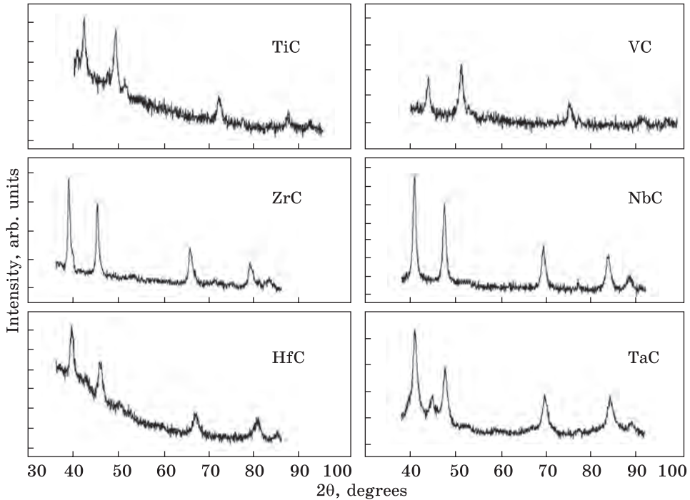
Fig. 11. XRD patterns of the milled Me-CNT charge after treatment by HCl and annealing at 700 °C, CoK _{\alpha} radiation
