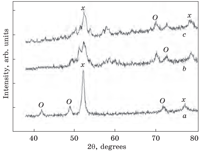
Fig. 27. Fragments of diffractograms for Fe-Ti-CNT samples consolidated via HP-HT method (CoK _{\alpha} radiation)
