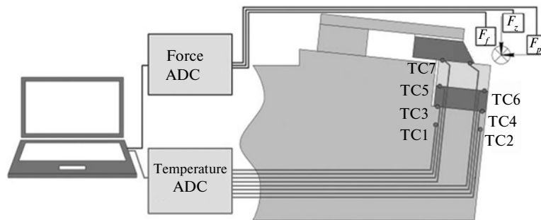
Fig. 1. Schematic view of the experimental setup.
