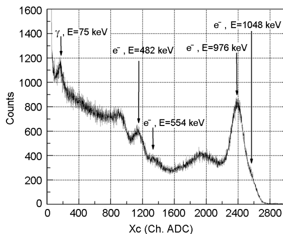
Fig. Energy spectrum for 207 Bi conversion electrons measured by the "SiPM- p -terphenyl" assembly.
