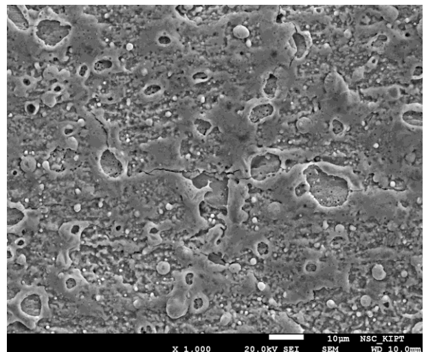
Fig. 2. SEM images of Ti-Cr-Ti-Zr coatings (irradiation with heat load of 0.6 MJ/m 2 )
