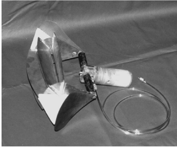
Fig. 6. Antenna design
