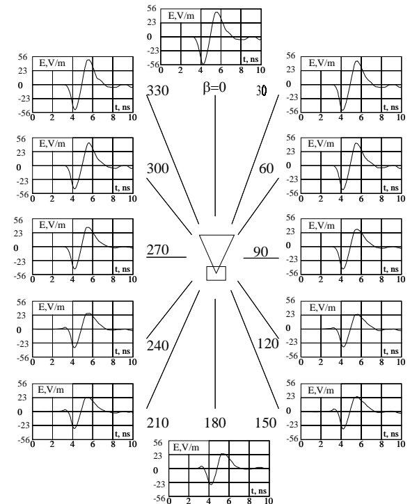
Fig. 8. Angular dependence of radiated pulses shape. H-plane
