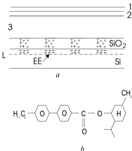
Fig. 4. a) Schematic view of the cholesteric cell based on the \text{Si}/\text{SiO}_2 structure. 1 – ITO electrode, 2 – rubbed polyimide layer for alignment of cholesteric, 3 – cholesteric layer, L – near-surface depletion boundary, EE – electron enrichment. b) Chiral component of cholesteric-nematic mixture.
