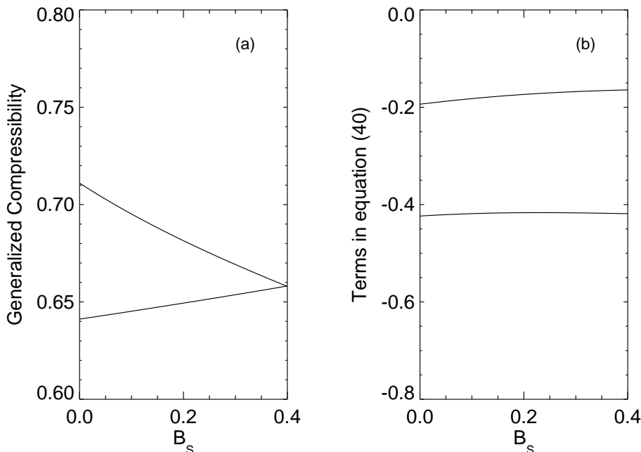
Figure 3. Sensitivity of two thermodynamic consistency tests with the bridge parameter B_S in the HNC/ \lambda_1 integral equation closure. The results shown correspond to a 2–2 aqueous electrolyte solution of concentration c_s = 0.02 \text{ mol dm}^{-3} at 298.15 K. (a) Generalized compressibility test: \beta(\partial\pi/\partial\rho_t)_T calculated according to the compressibility route (upper curve) and the virial route (lower curve). (b) Maxwell relation derived test: (energy route)-based left hand side of equation (42) (lower curve) and (compressibility route)-based right hand side of equation (42) (upper curve).
