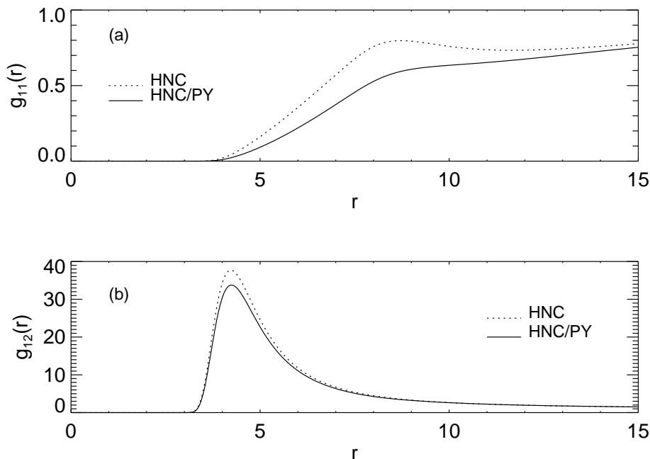
Figure 1. Ion-ion radial distribution functions for an aqueous solution of a restricted 2–2 electrolyte at c_s = 0.02 \text{ mol dm}^{-3} and 298.15 K. The correlation functions are calculated under the integral equation closures HNC and HNC/PY. (a): Like-sign (cation-cation or anion-anion) correlation function g_{11}(r) ; (b): cation-anion correlation function g_{12}(r) . r is in units of Å.
