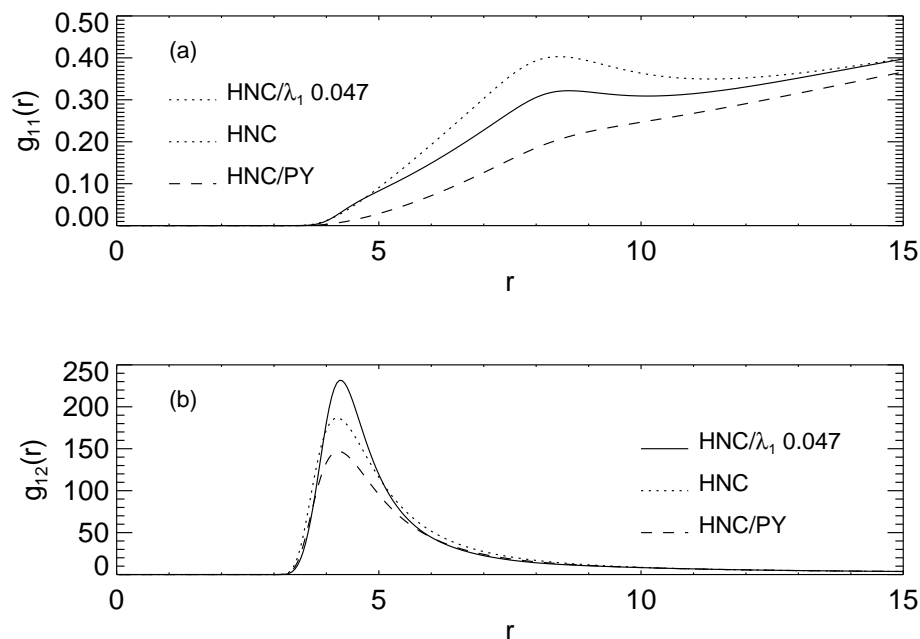
Figure 5. Ion-ion radial distribution functions for an aqueous solution of a restricted 2–2 electrolyte at c_s = 0.001 \text{ mol dm}^{-3} and 298.15 K. The correlation functions are calculated under the integral equation closures HNC, HNC/PY, and HNC/ \lambda_1 with the bridge parameter B_S = 0.047 , for which u_{\text{HNC}/\lambda_1} = u_{\text{HNC}} . (a): Like-sign (cation-cation or anion-anion) correlation function g_{11}(r) ; (b): cation-anion correlation function g_{12}(r) . r is in units of \text{\AA} .
