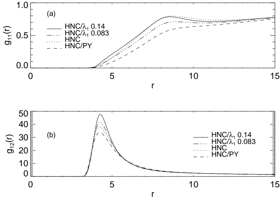
Figure 4. Ion-ion radial distribution functions for an aqueous solution of a restricted 2–2 electrolyte at c_s = 0.02 \text{ mol dm}^{-3} and 298.15 K. The correlation function are calculated under the integral equation closures HNC, HNC/PY, and HNC/ \lambda_1 for two values of the bridge parameter B_S . These are B_S = 0.14 , when (g_{12}^{\text{max}})_{\text{HNC}/\lambda_1} = (g_{12}^{\text{max}})_{\text{HNC}} , and B_S = 0.083 , when u_{\text{HNC}/\lambda_1} = u_{\text{HNC}} . (a): Like-sign (cation-cation or anion-anion) correlation function g_{11}(r) ; (b): cation-anion correlation function g_{12}(r) . r is in units of Å.
