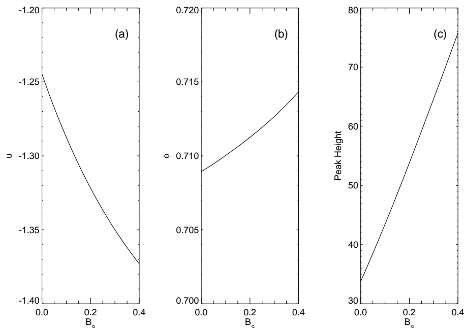
Figure 2. Dependence of thermodynamic and structural properties of an electrolyte solution with the bridge parameter B_S under closure HNC/ \lambda_1 . The results shown correspond to a 2–2 aqueous electrolyte solution of concentration c_s = 0.02 \text{ mol dm}^{-3} at 298.15 K. (a) Reduced excess internal energy per ion, u , calculated with equation (37); (b) osmotic coefficient \phi , calculated with equation (38); (c) peak height g_{12}^{\text{max}} in the cation-anion pair correlation function g_{12}(r) .
