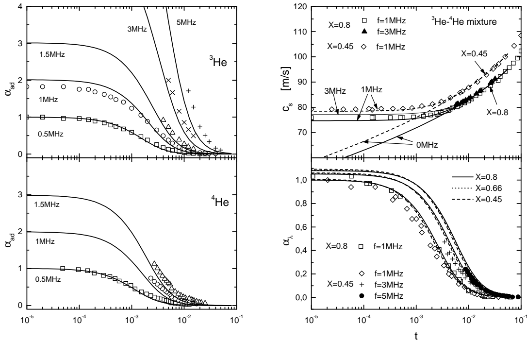
Figure 3. Sound attenuation for (a) pure He (from [5]) and sound velocity and sound attenuation for mixtures (from [6]).
