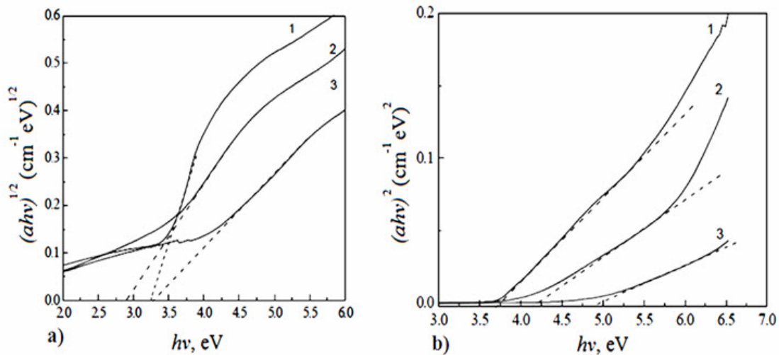
Fig. 2. Bandgap widths E_{gi} for indirect (a) and E_{gd} for direct (b) transitions in nanocomposites of TiO 2 (1), TiO 2 /ZrO 2 (2), TiO 2 /ZrO 2 /SiO 2 (3).
