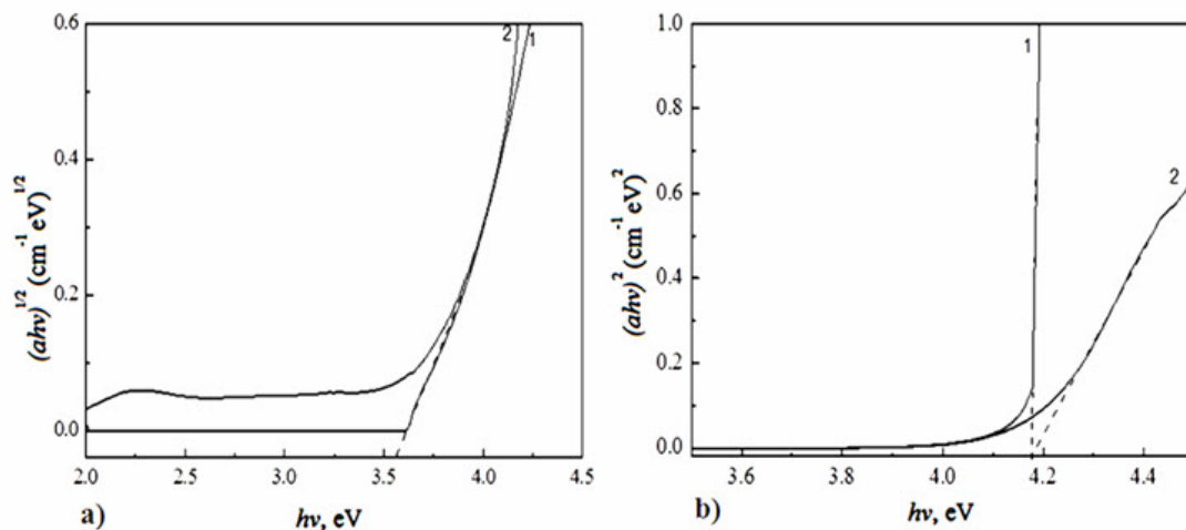
Fig. 3. Bandgap widths E_{gi} for indirect (a) and E_{gd} for direct (b) transitions in nanocomposites of TiO 2 /ZrO 2 /SiO 2 /Ag (1), TiO 2 /ZrO 2 /SiO 2 /Au (2).
