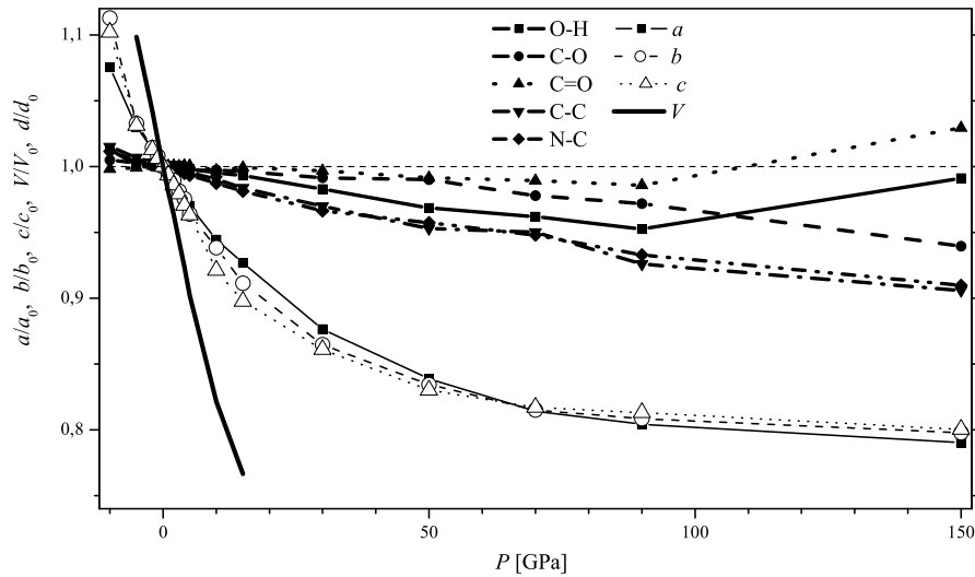
Figure 1. Pressure dependencies of the relative unit cell parameters a/a_0 , b/b_0 , c/c_0 , V/V_0 , and interatomic distances d/d_0 of the glycine group of TGS crystal.
