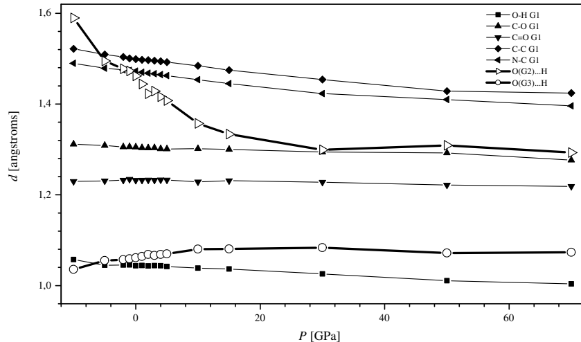
Figure 2. Pressure dependencies of the interatomic distances d of the glycine group G1 and hydrogen bond O(G2)–H...O(G3) of TGS crystal.
