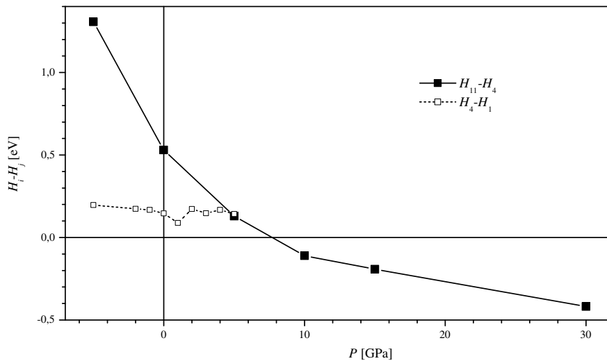
Figure 3. Dependencies of the difference of enthalpies H_i - H_j on the hydrostatic pressure P for the space groups 11 ( P2_1/m ), 4 ( P2_1 ) and 1 ( P1 ) of TGS crystal.
