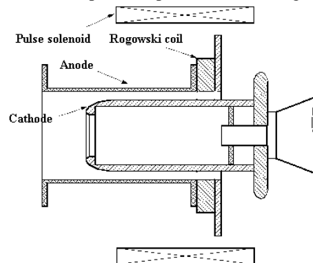
Fig. 2. The gun design for nanosecond mode
