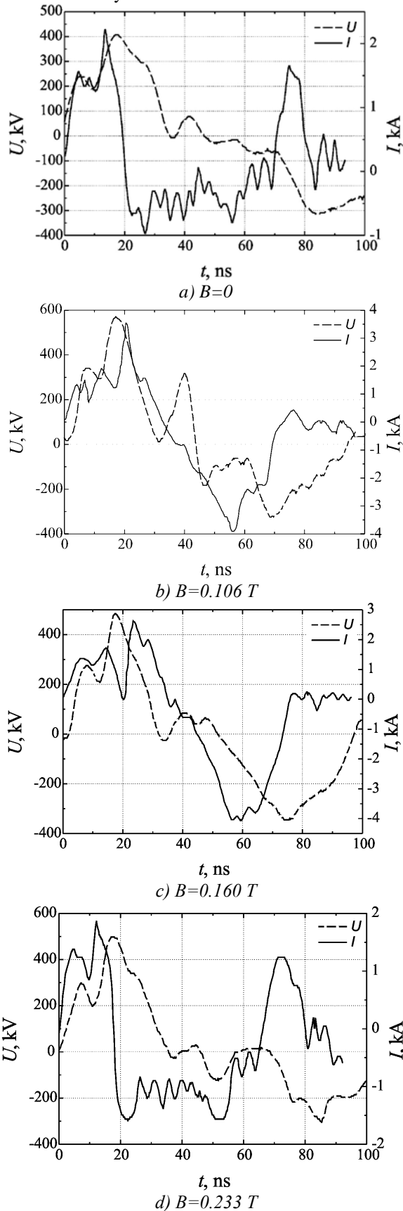
Fig. 5. Synchronous oscillograms of the gun current and voltage at different values of a magnetic field B are shown. The charge voltage of the Marx generator was 32 kV
