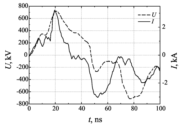
Fig. 6. Synchronous oscillograms of the gun current and voltage at a magnetic field B=0.266 T are shown. The charge voltage of the Marx generator was 40 kV
