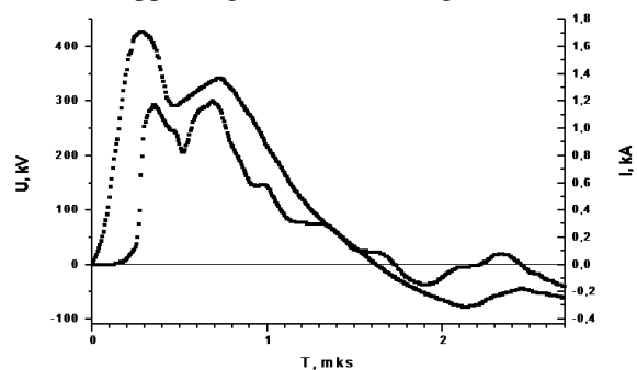
Fig. 3. Gun voltage (first, up) and beam current (second, down) at magnetic field B=0.34 T at the microsecond output
