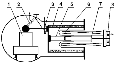
Fig. 1. Scheme of the microsecond output with SEMIG:
