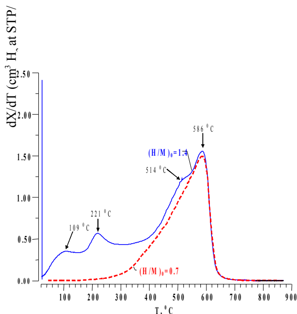
Fig.2. The thermal desorption spectrum of hydrogen from ZrV_2H_x samples with various initial concentrations of hydrogen
