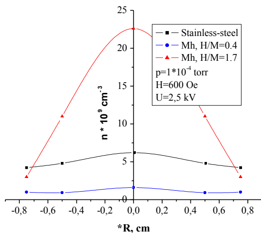
Fig.4. The radial distribution of plasma density in the reflective discharge
