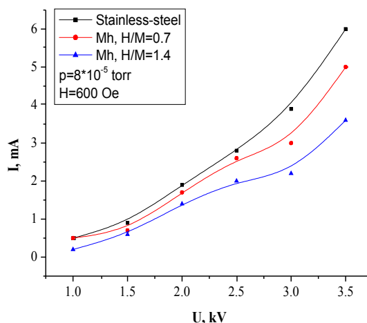
Fig. 3 The current-voltage characteristics of the reflective discharge
