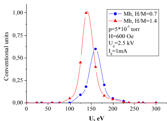
Fig.5. The energy distribution of the paraxial ion group in the reflective discharge
