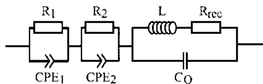
Fig. 2. The equivalent electric circuit.
